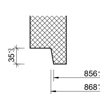
Detail Spitzende, 1:5
