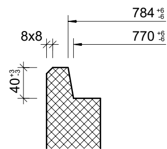
Detail Muffe, 1:5
