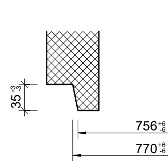
Detail Spitzende, 1:5
