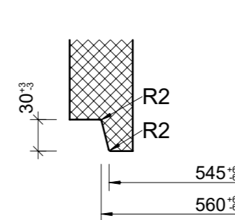
Detail Spitzende, 1:5
