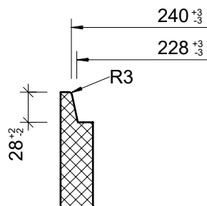
Detail Muffe, 1:5
