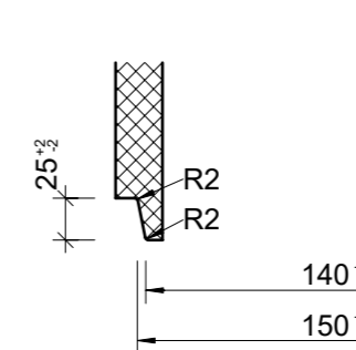
Detail Spitzende, 1:5
