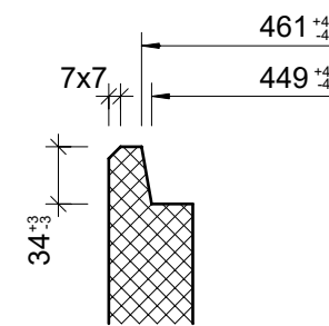
Detail Muffe, 1:5
