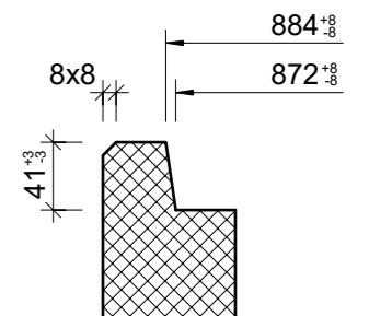
Detail Muffe, 1:5
