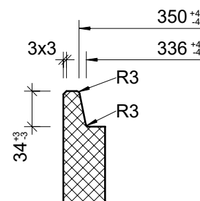
Detail Muffe, 1:5
