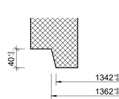
Detail Spitzende, 1:5
