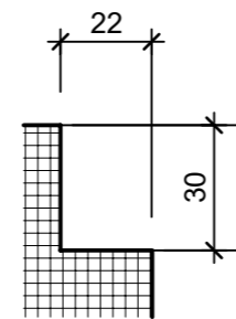
Detail A 1:2
