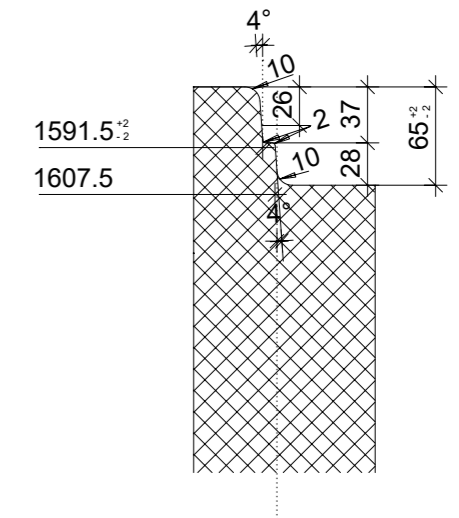
Zapfendetail, 1:5
