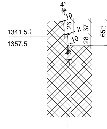
Zapfendetail, 1:5
