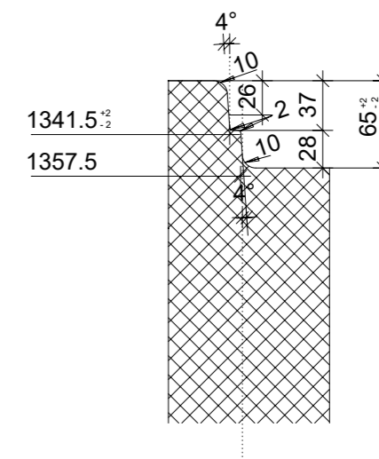
Zapfendetail, 1:5
