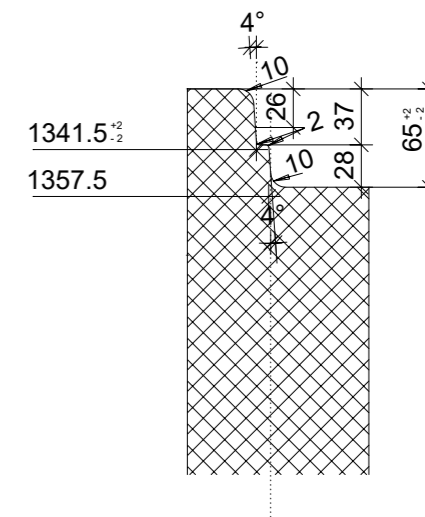
Zapfendetail, 1:5
