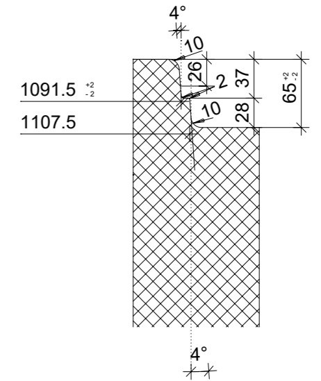
Zapfendetail, 1:5
