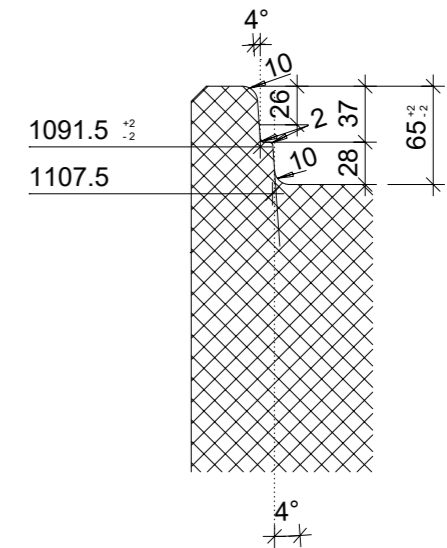
Zapfendetail, 1:5
