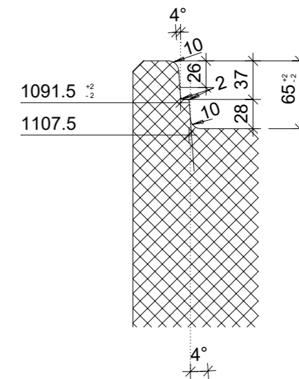
Zapfendetail, 1:5
