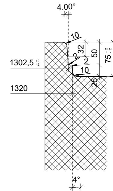
Zapfendetail, 1:5
